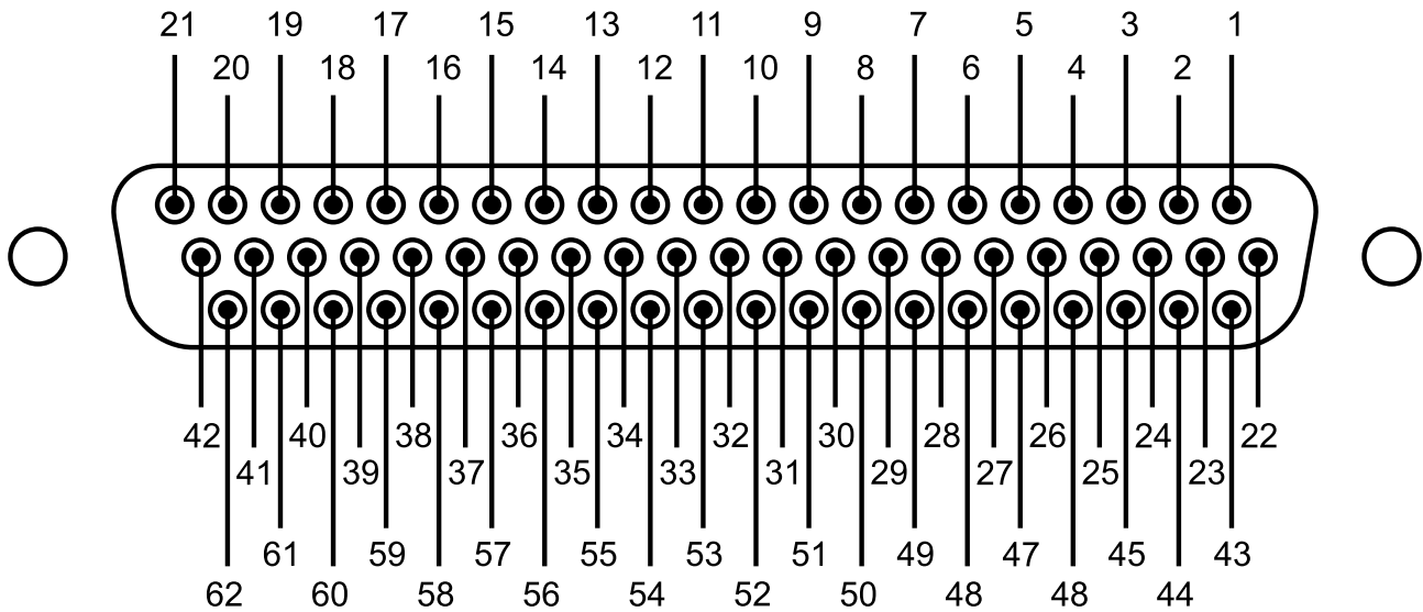
DB62 Female
